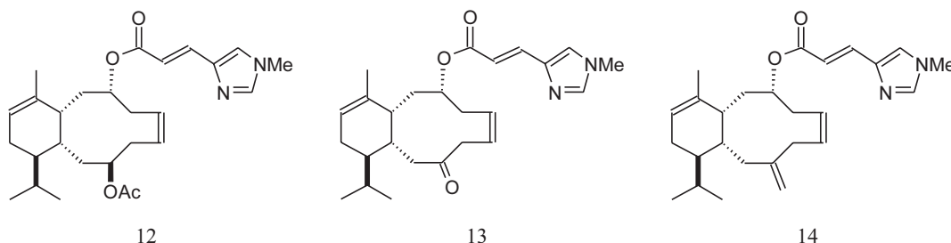
Fig. 2. Eleutheside analogues 12–14
