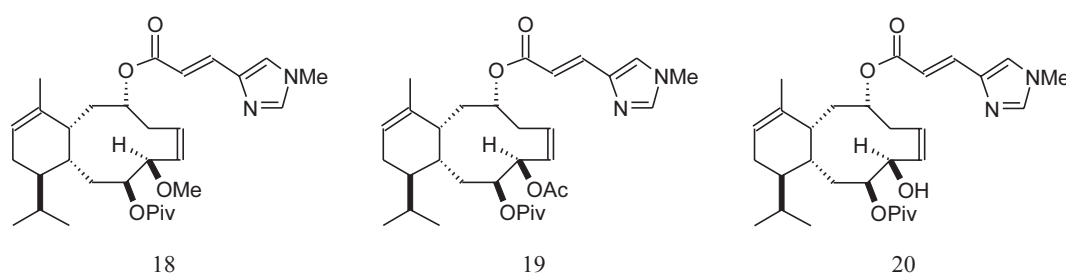
Fig. 3. Eleutheside analogues 18–20
