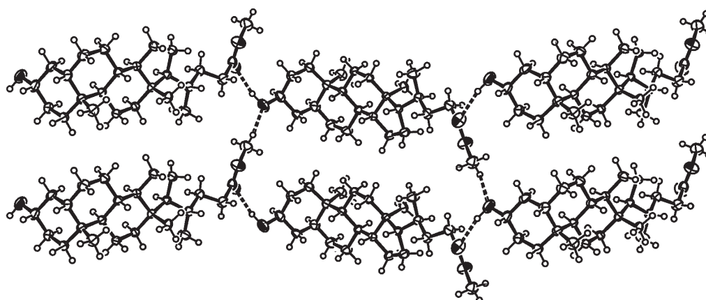
Fig. 4. Crystal packing of methyl lithocholate showing head-to-tail intermolecular hydrogen bonding between C 24 = O...H-O-C 3 and one proton of the ester methyl CH 3 ...O-C 3 with the other molecule in the adjacent polymeric steroidal chain
