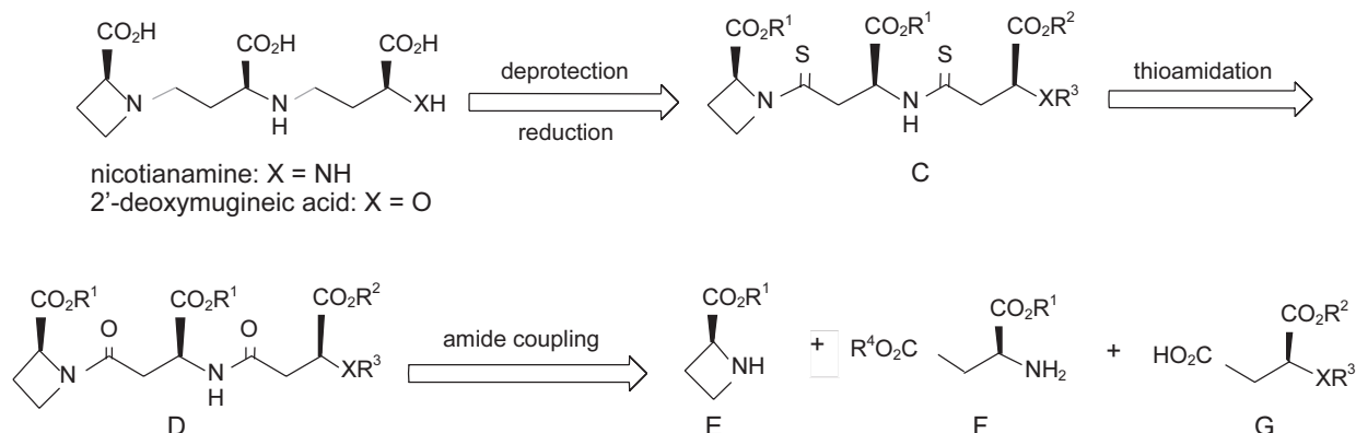
Fig. 4. Retrosynthesis of Phytosiderophores
