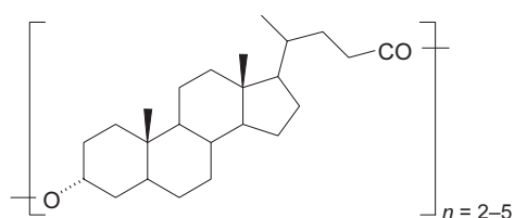
Fig. 2. Structures of dimeric to pentameric cyclolithocholates
