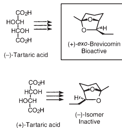
Fig. 1. Synthesis of the enantiomers of exo -brevicommin
